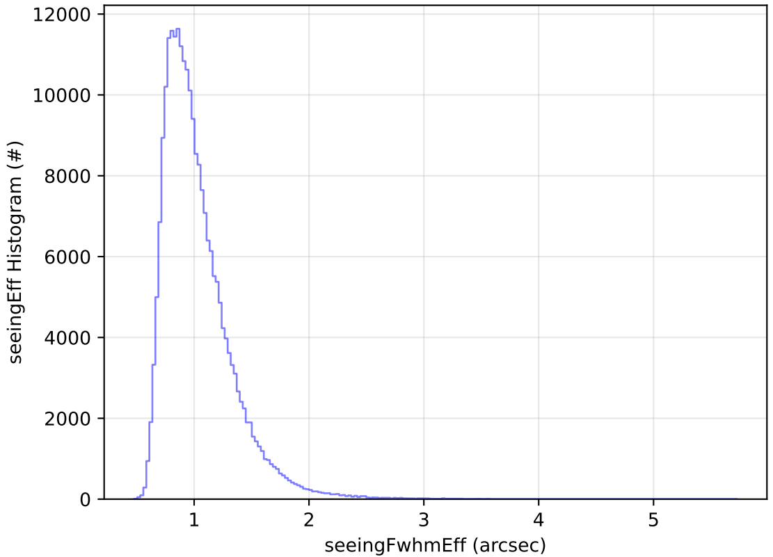
early_ss_template_fpextra2.0_v3.4_10yrs Yr 1 all bands: seeingEff Histogram
