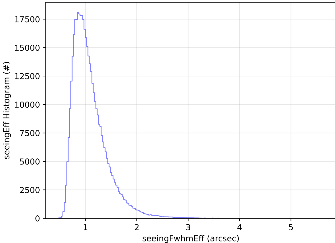
early_ss_template_fpextra2.0_v3.4_10yrs WFD z band: seeingEff Histogram
