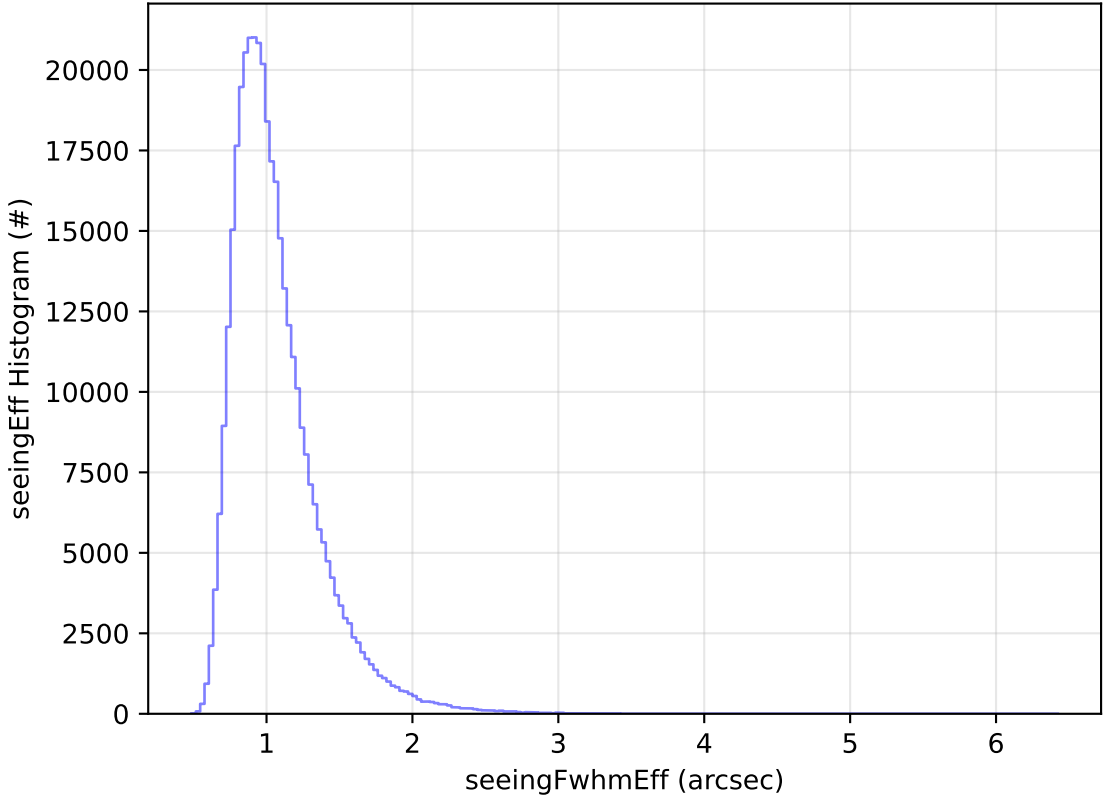
early_ss_template_fpextra2.0_v3.4_10yrs WFD y band: seeingEff Histogram
