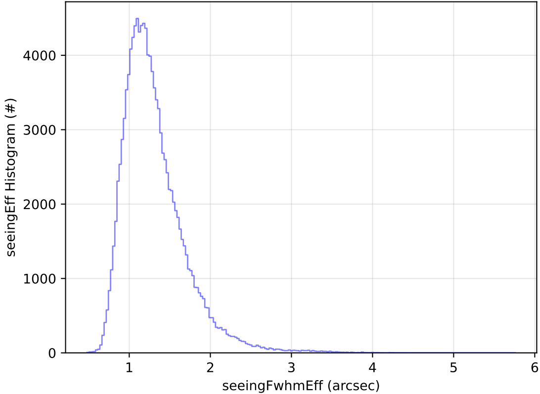
early_ss_template_fpextra2.0_v3.4_10yrs WFD u band: seeingEff Histogram
