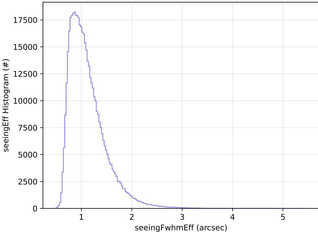
early_ss_template_fpextra2.0_v3.4_10yrs WFD r band: seeingEff Histogram
