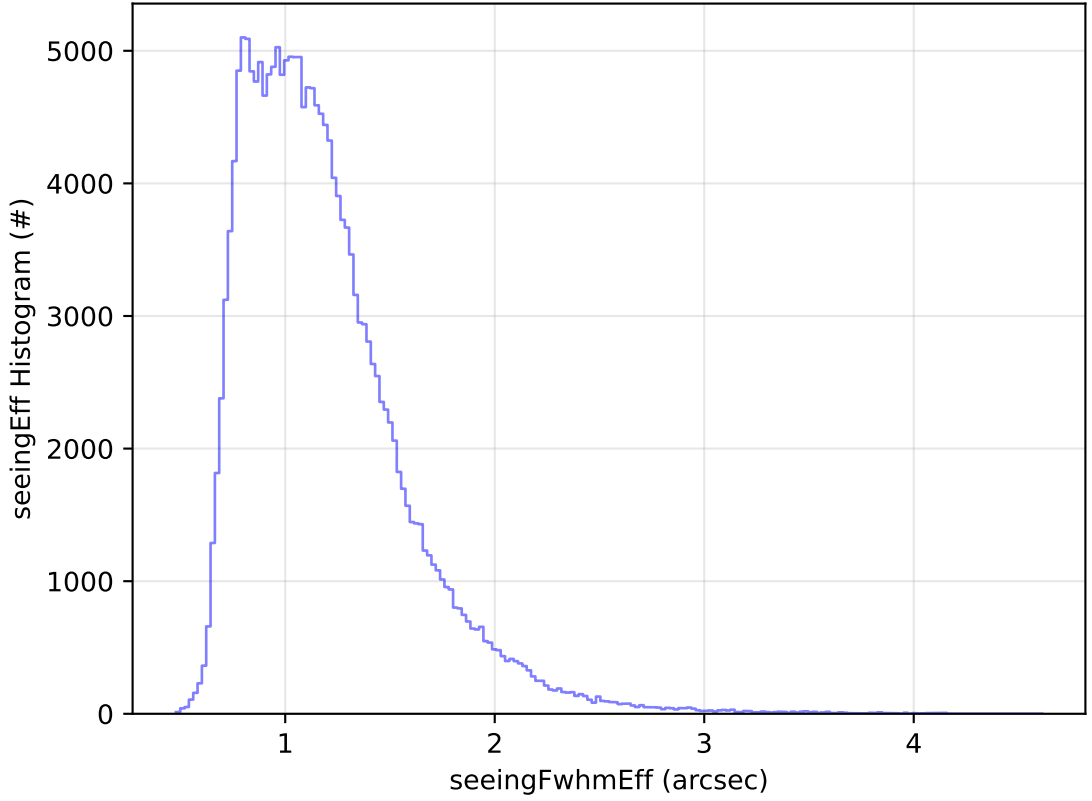
early_ss_template_fpextra2.0_v3.4_10yrs WFD g band: seeingEff Histogram
