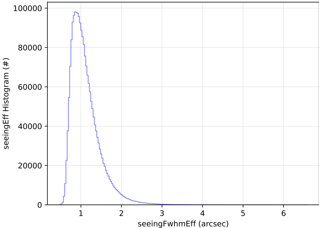
early_ss_template_fpextra2.0_v3.4_10yrs WFD all bands: seeingEff Histogram
