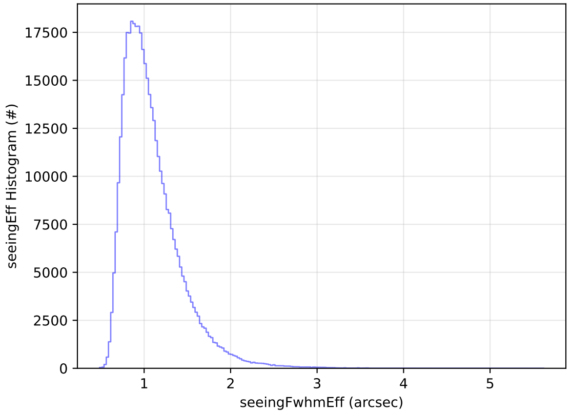
early_ss_template_fpextra2.0_v3.4_10yrs All sky z band: seeingEff Histogram
