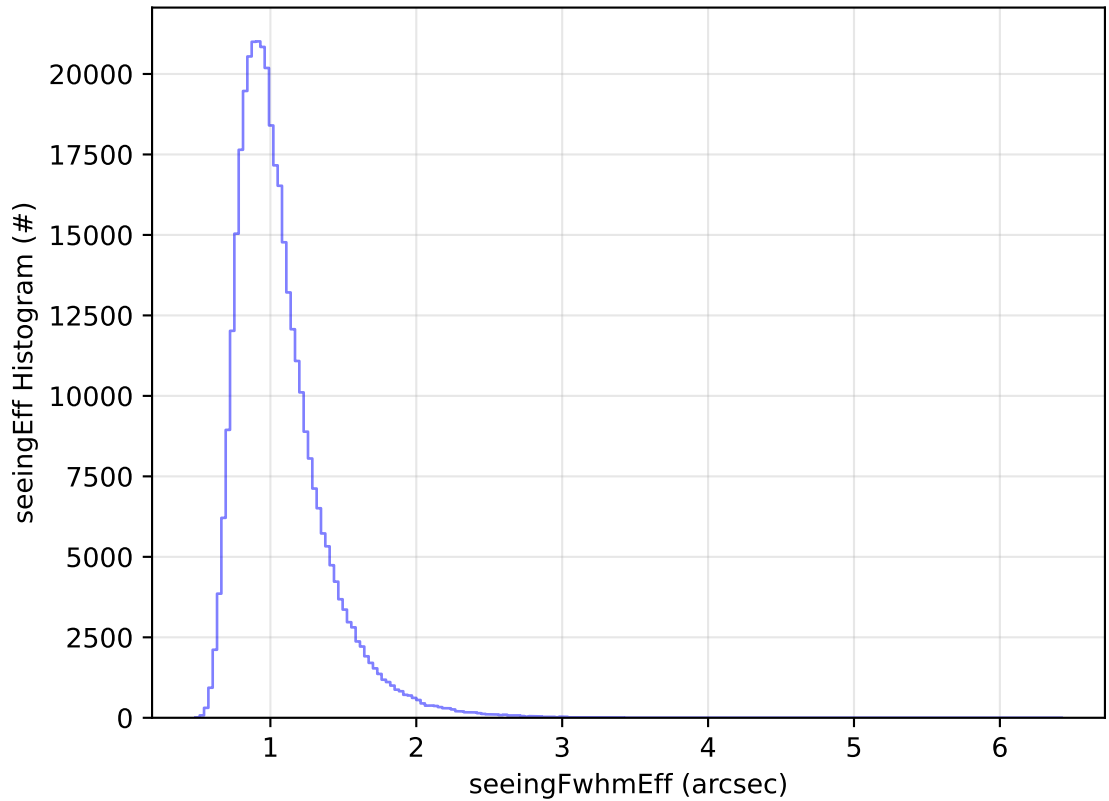
early_ss_template_fpextra2.0_v3.4_10yrs All sky y band: seeingEff Histogram
