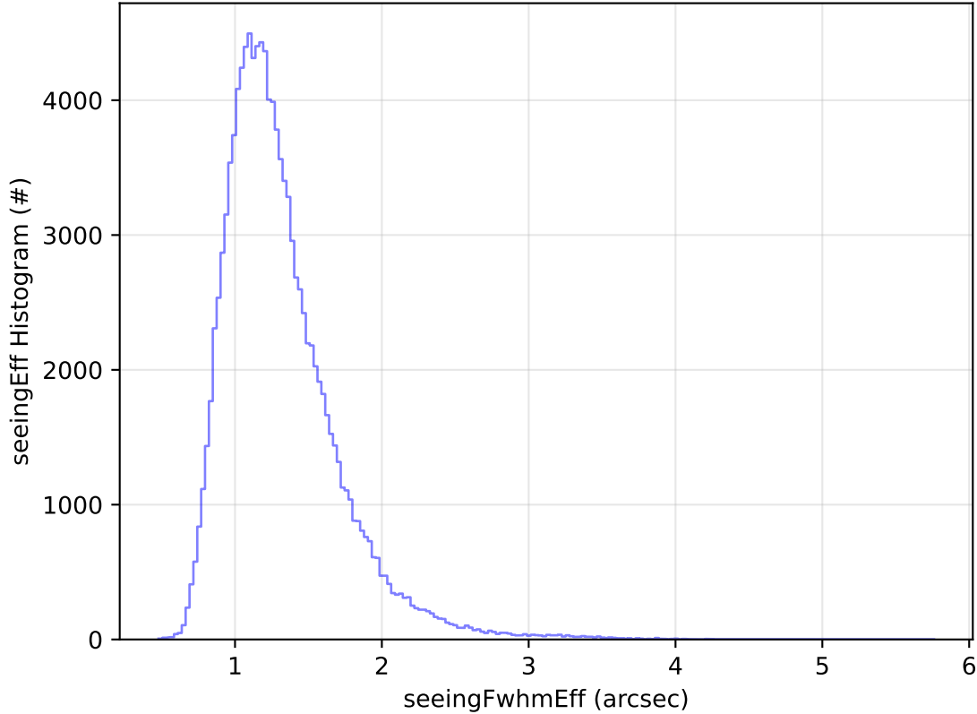
early_ss_template_fpextra2.0_v3.4_10yrs All sky u band: seeingEff Histogram
