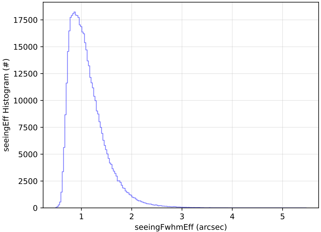
early_ss_template_fpextra2.0_v3.4_10yrs All sky r band: seeingEff Histogram
