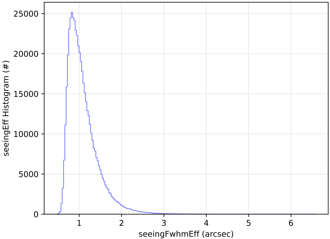
early_ss_template_fpextra2.0_v3.4_10yrs All sky i band: seeingEff Histogram
