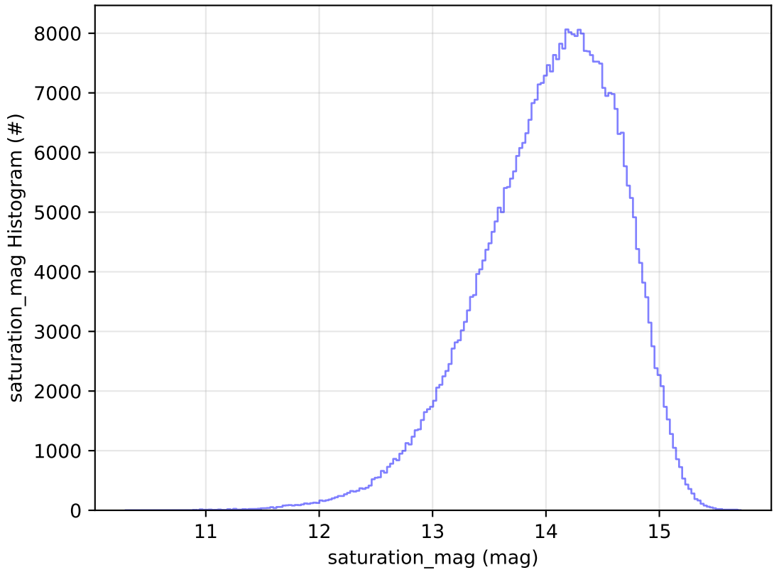
early_ss_template_fpextra2.0_v3.4_10yrs WFD z band: saturation_mag Histogram
