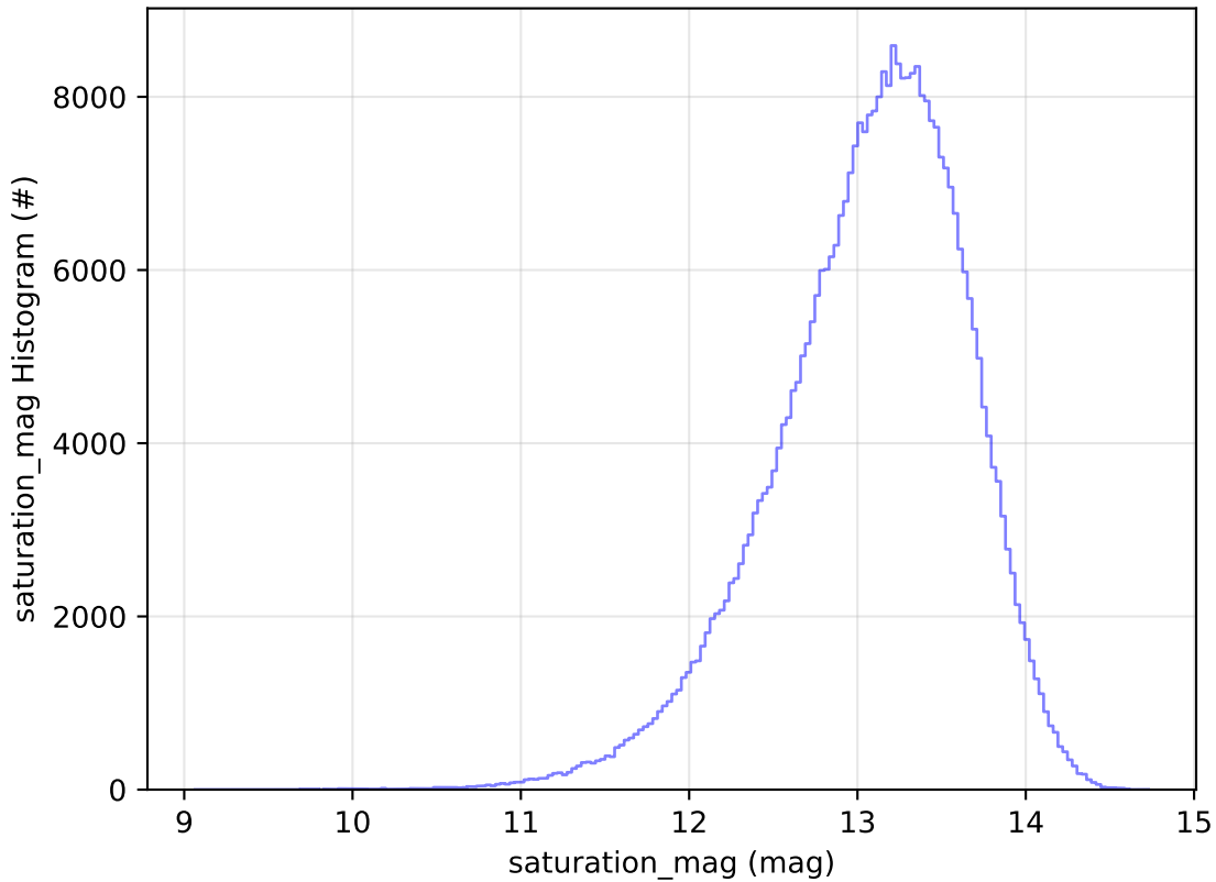
early_ss_template_fpextra2.0_v3.4_10yrs WFD y band: saturation_mag Histogram
