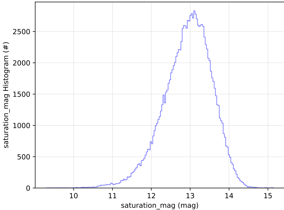
early_ss_template_fpextra2.0_v3.4_10yrs WFD u band: saturation_mag Histogram
