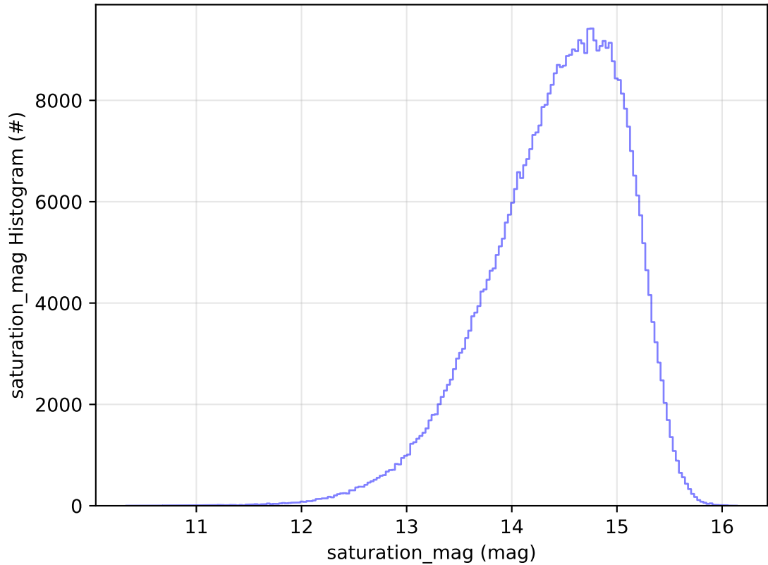
early_ss_template_fpextra2.0_v3.4_10yrs WFD i band: saturation_mag Histogram
