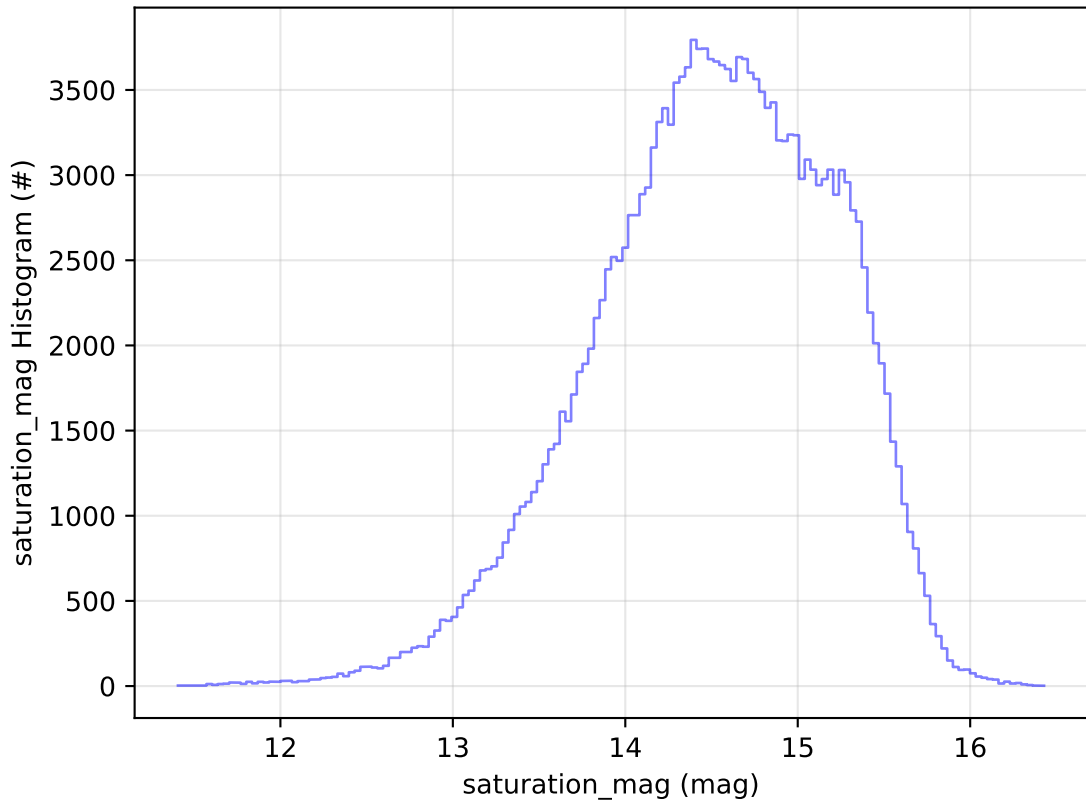
early_ss_template_fpextra2.0_v3.4_10yrs WFD g band: saturation_mag Histogram
