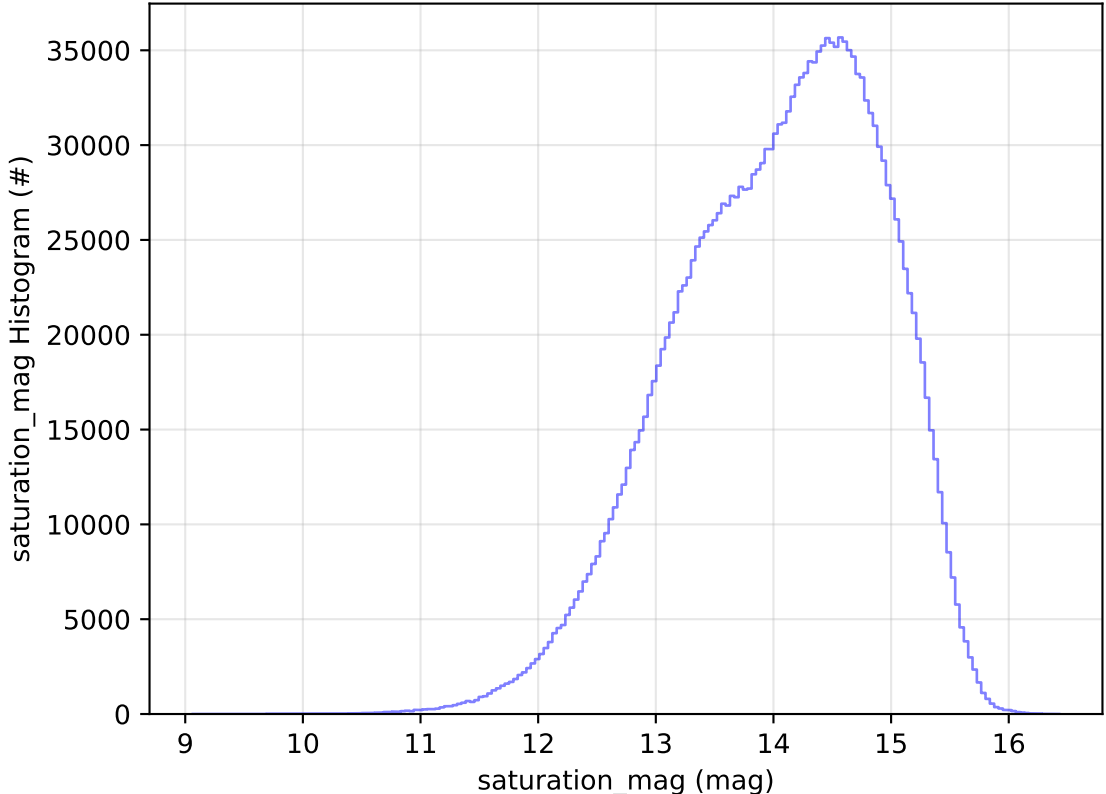
early_ss_template_fpextra2.0_v3.4_10yrs WFD all bands: saturation_mag Histogram
