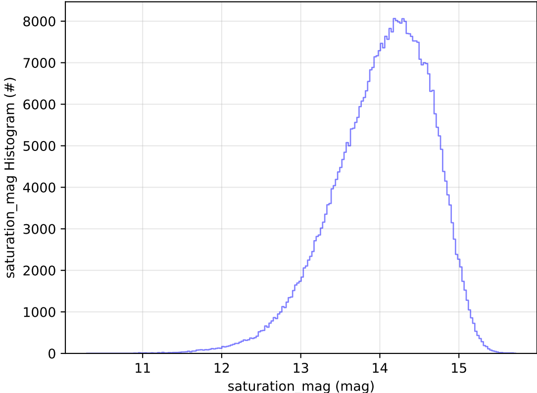
early_ss_template_fpextra2.0_v3.4_10yrs All sky z band: saturation_mag Histogram
