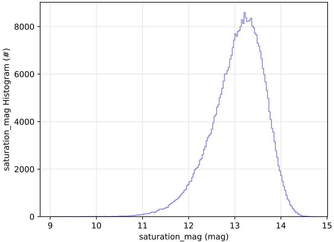
early_ss_template_fpextra2.0_v3.4_10yrs All sky y band: saturation_mag Histogram
