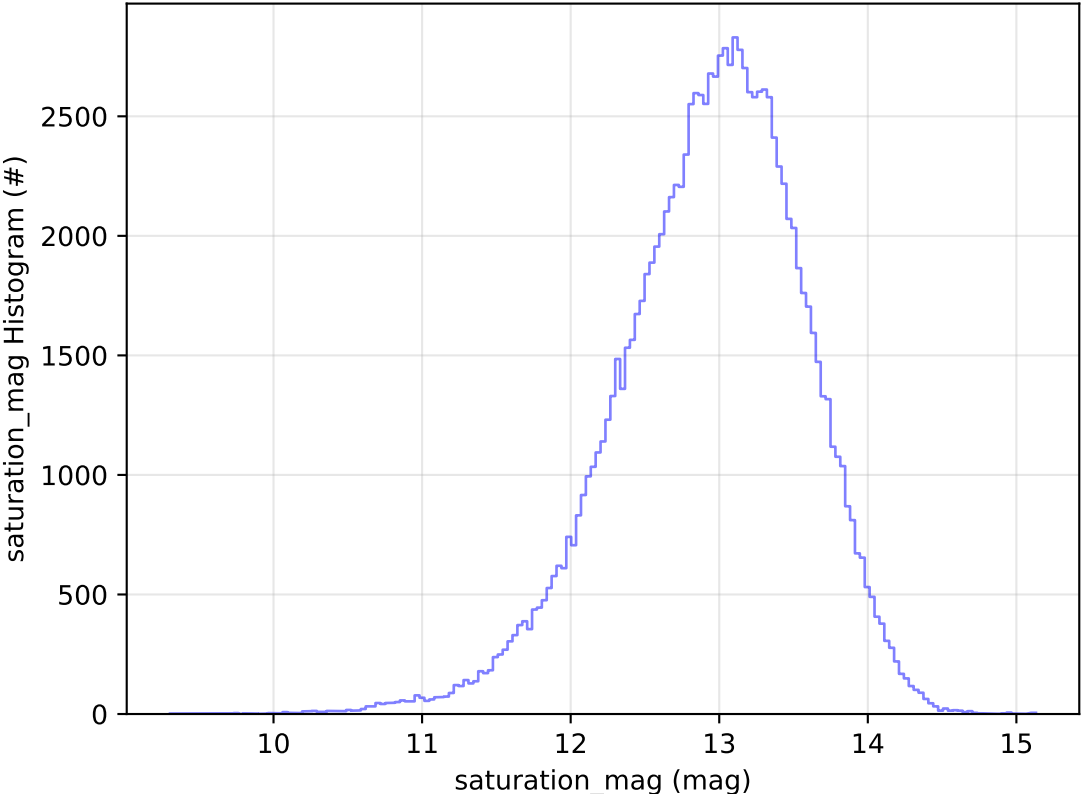
early_ss_template_fpextra2.0_v3.4_10yrs All sky u band: saturation_mag Histogram
