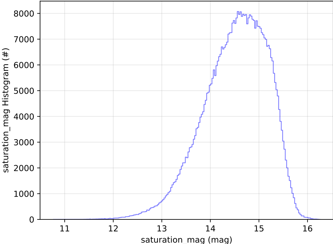
early_ss_template_fpextra2.0_v3.4_10yrs All sky r band: saturation_mag Histogram
