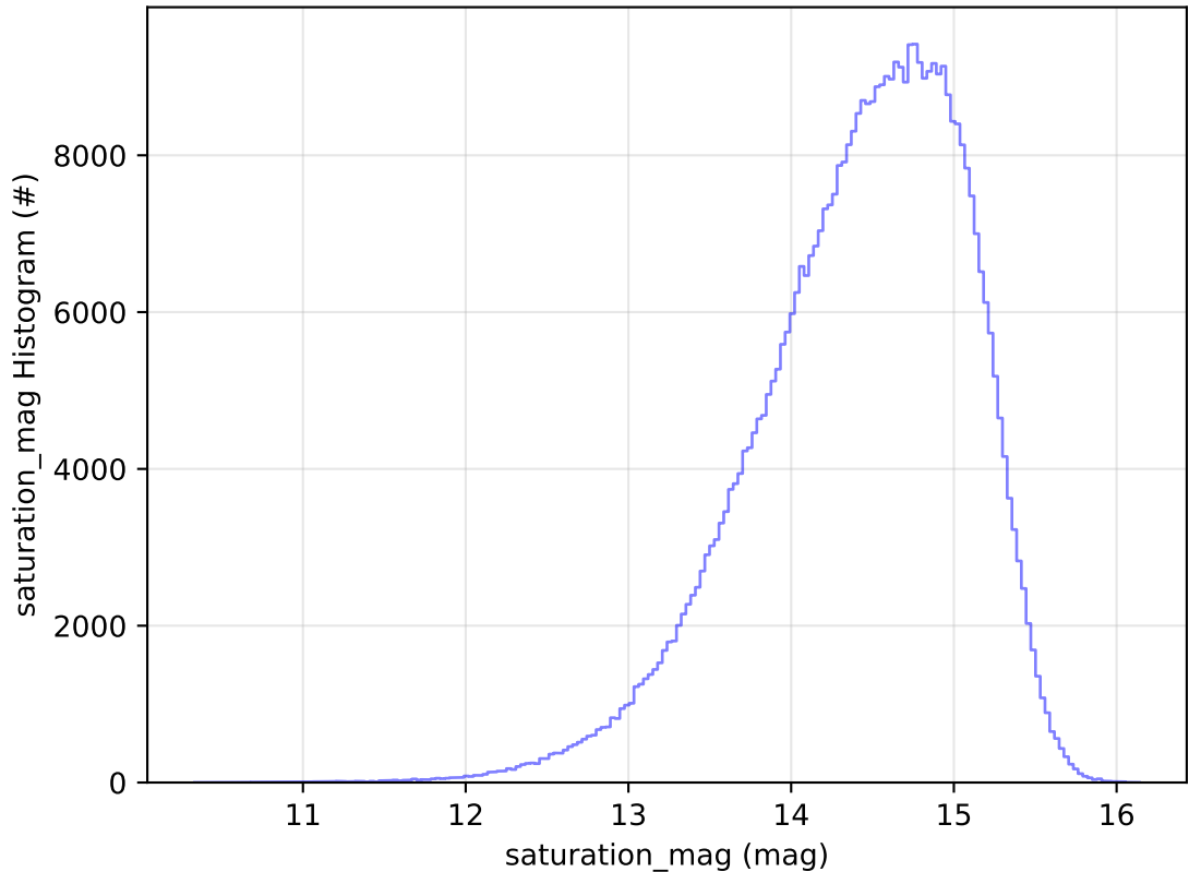
early_ss_template_fpextra2.0_v3.4_10yrs All sky i band: saturation_mag Histogram
