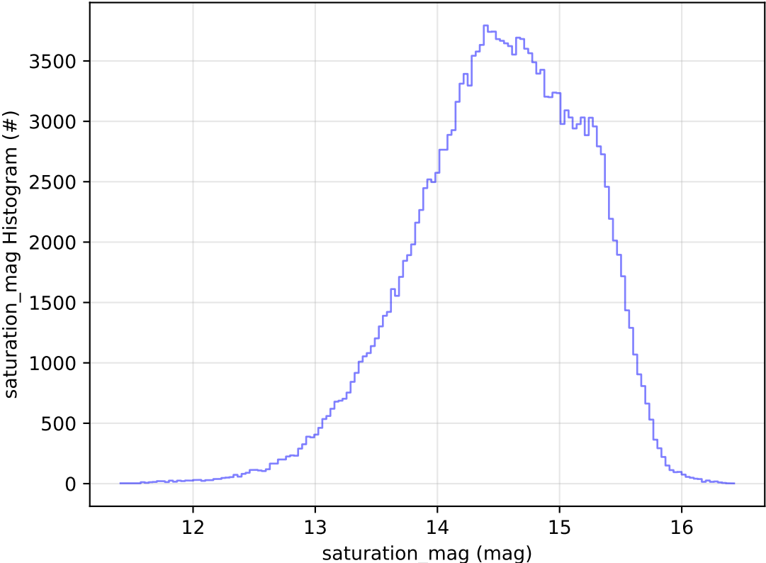
early_ss_template_fpextra2.0_v3.4_10yrs All sky g band: saturation_mag Histogram
