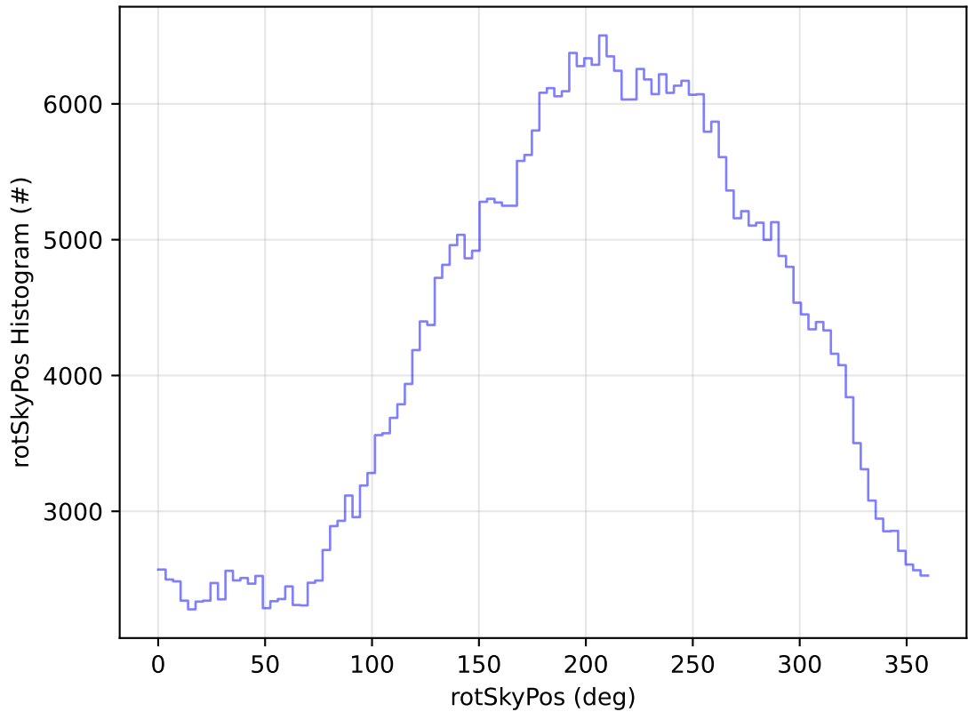
early_ss_template_fpextra2.0_v3.4_10yrs WFD z band: rotSkyPos Histogram
