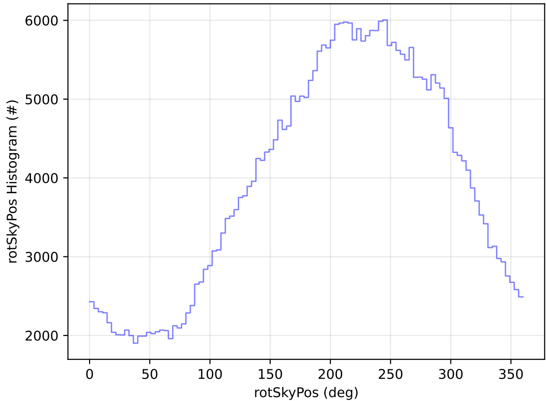
early_ss_template_fpextra2.0_v3.4_10yrs WFD y band: rotSkyPos Histogram
