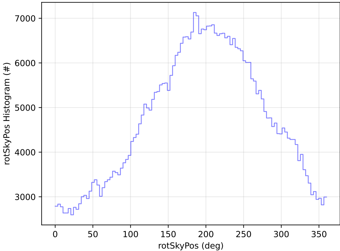
early_ss_template_fpextra2.0_v3.4_10yrs WFD r band: rotSkyPos Histogram
