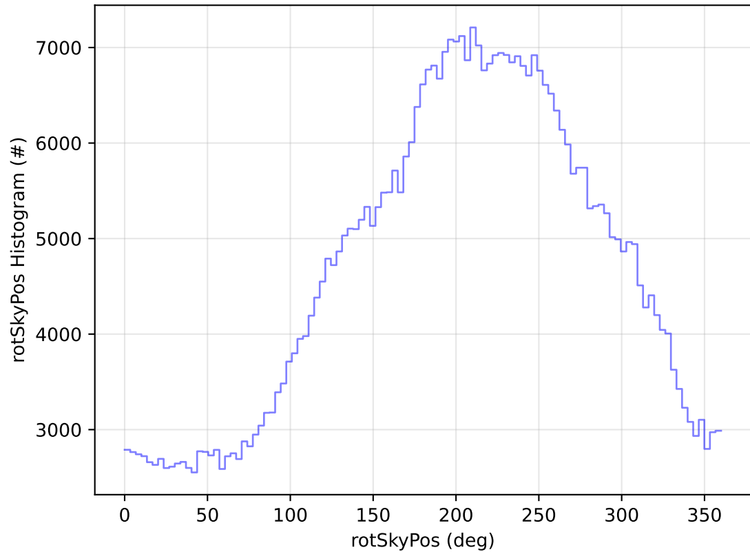
early_ss_template_fpextra2.0_v3.4_10yrs WFD i band: rotSkyPos Histogram
