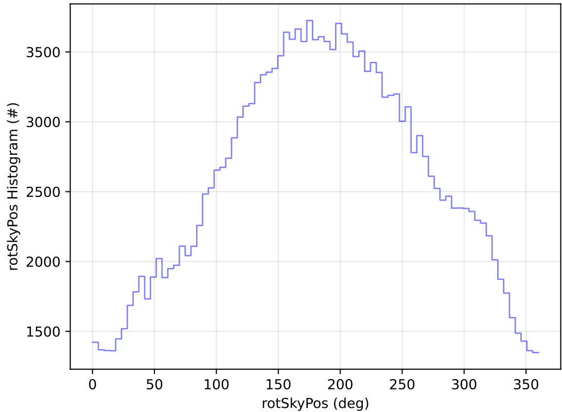
early_ss_template_fpextra2.0_v3.4_10yrs WFD g band: rotSkyPos Histogram
