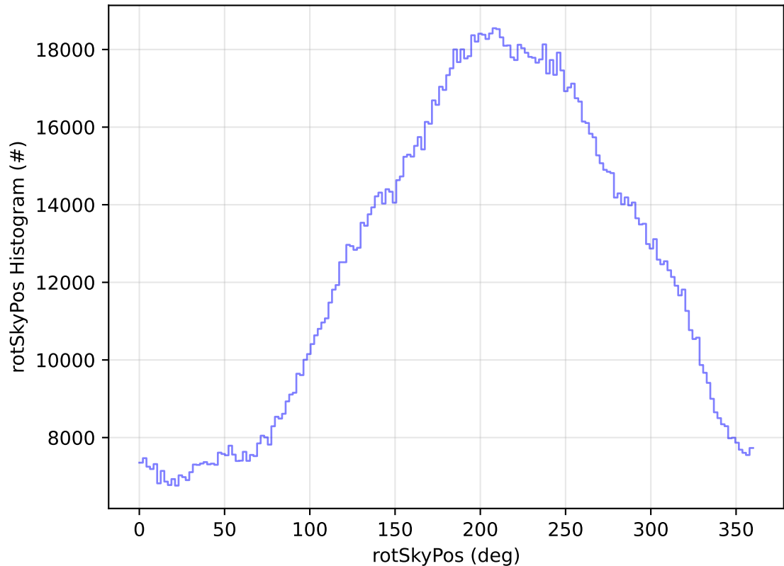
early_ss_template_fpextra2.0_v3.4_10yrs WFD all bands: rotSkyPos Histogram
