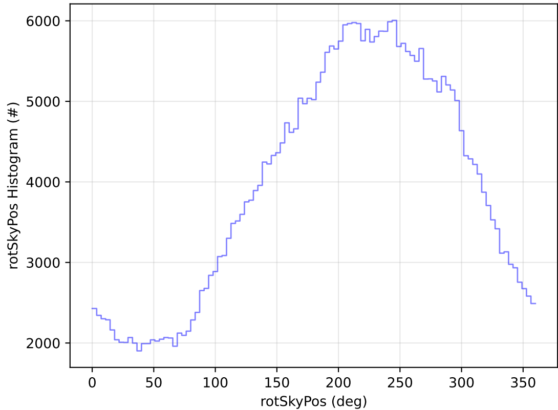
early_ss_template_fpextra2.0_v3.4_10yrs All sky y band: rotSkyPos Histogram
