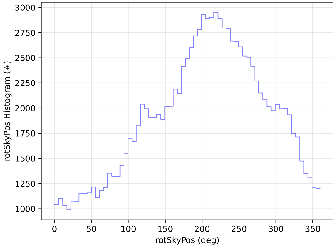
early_ss_template_fpextra2.0_v3.4_10yrs All sky u band: rotSkyPos Histogram
