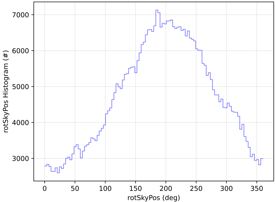
early_ss_template_fpextra2.0_v3.4_10yrs All sky r band: rotSkyPos Histogram
