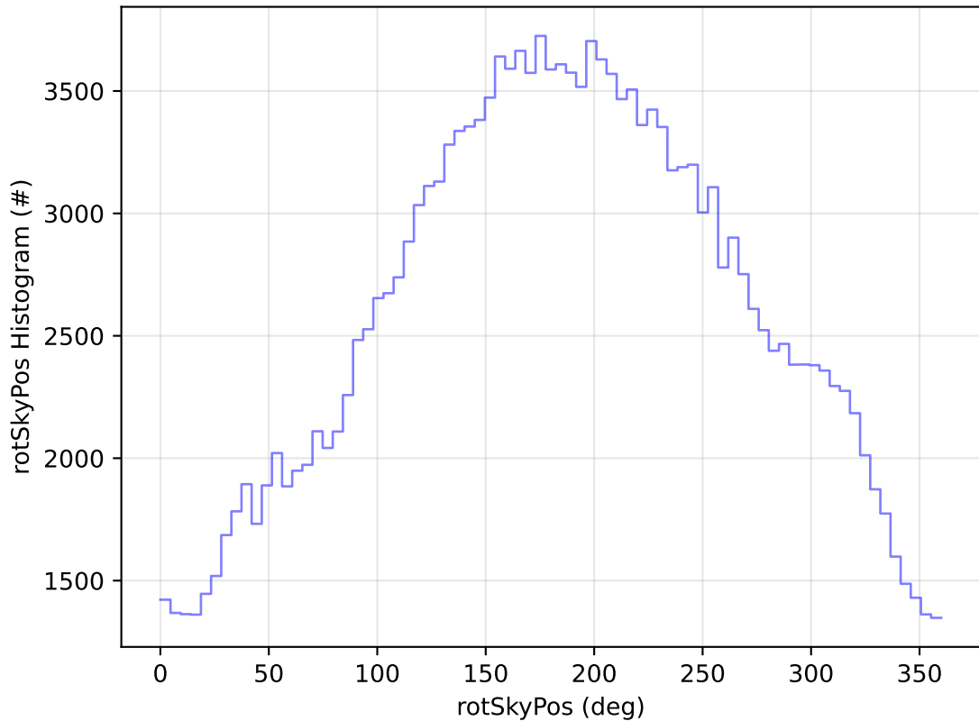
early_ss_template_fpextra2.0_v3.4_10yrs All sky g band: rotSkyPos Histogram
