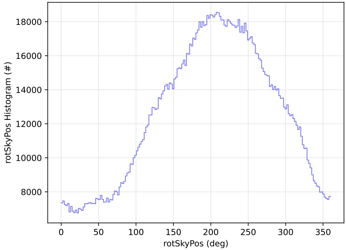
early_ss_template_fpextra2.0_v3.4_10yrs All sky all bands: rotSkyPos Histogram
