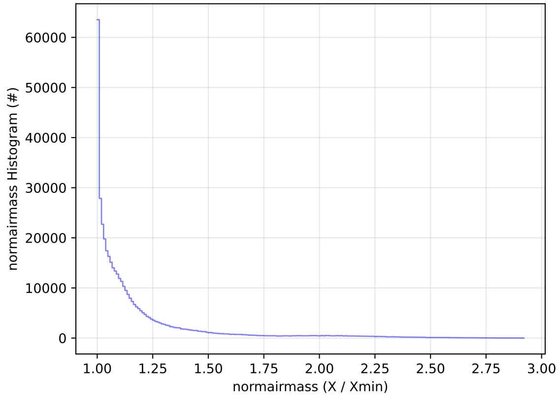
early_ss_template_fpextra2.0_v3.4_10yrs WFD z band: normairmass Histogram
