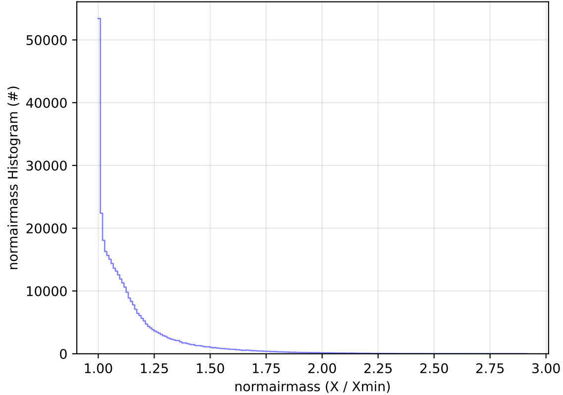
early_ss_template_fpextra2.0_v3.4_10yrs WFD y band: normairmass Histogram
