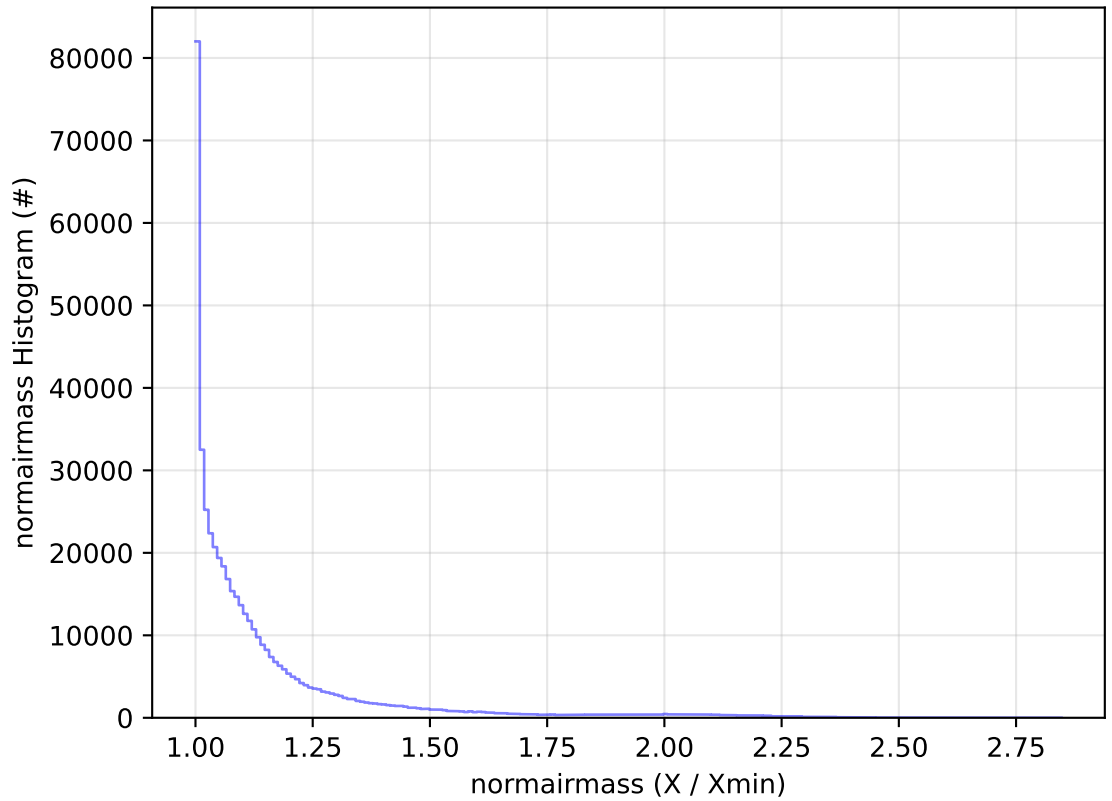
early_ss_template_fpextra2.0_v3.4_10yrs WFD r band: normairmass Histogram
