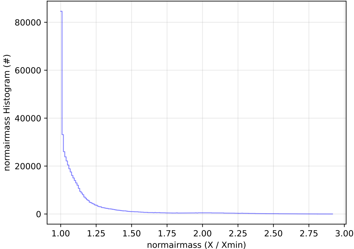
early_ss_template_fpextra2.0_v3.4_10yrs WFD i band: normairmass Histogram
