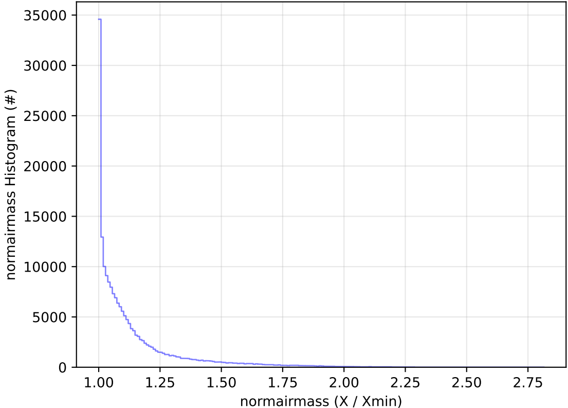
early_ss_template_fpextra2.0_v3.4_10yrs WFD g band: normairmass Histogram
