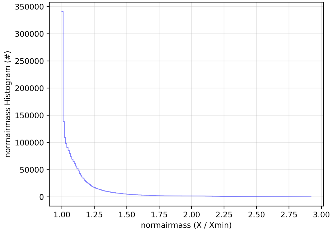
early_ss_template_fpextra2.0_v3.4_10yrs WFD all bands: normairmass Histogram
