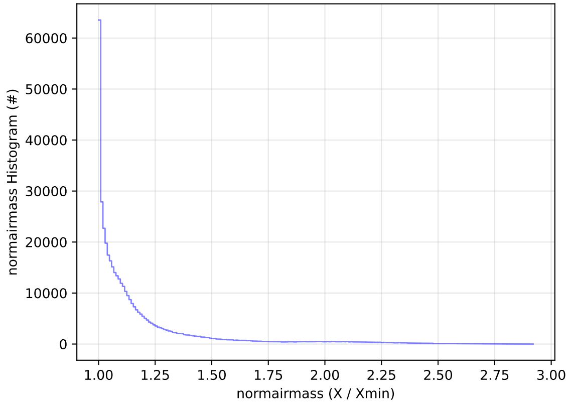
early_ss_template_fpextra2.0_v3.4_10yrs All sky z band: normairmass Histogram
