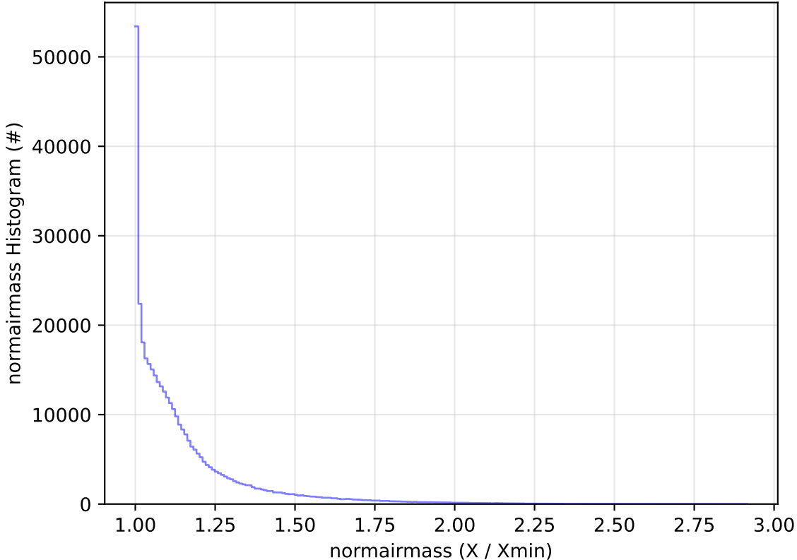
early_ss_template_fpextra2.0_v3.4_10yrs All sky y band: normairmass Histogram
