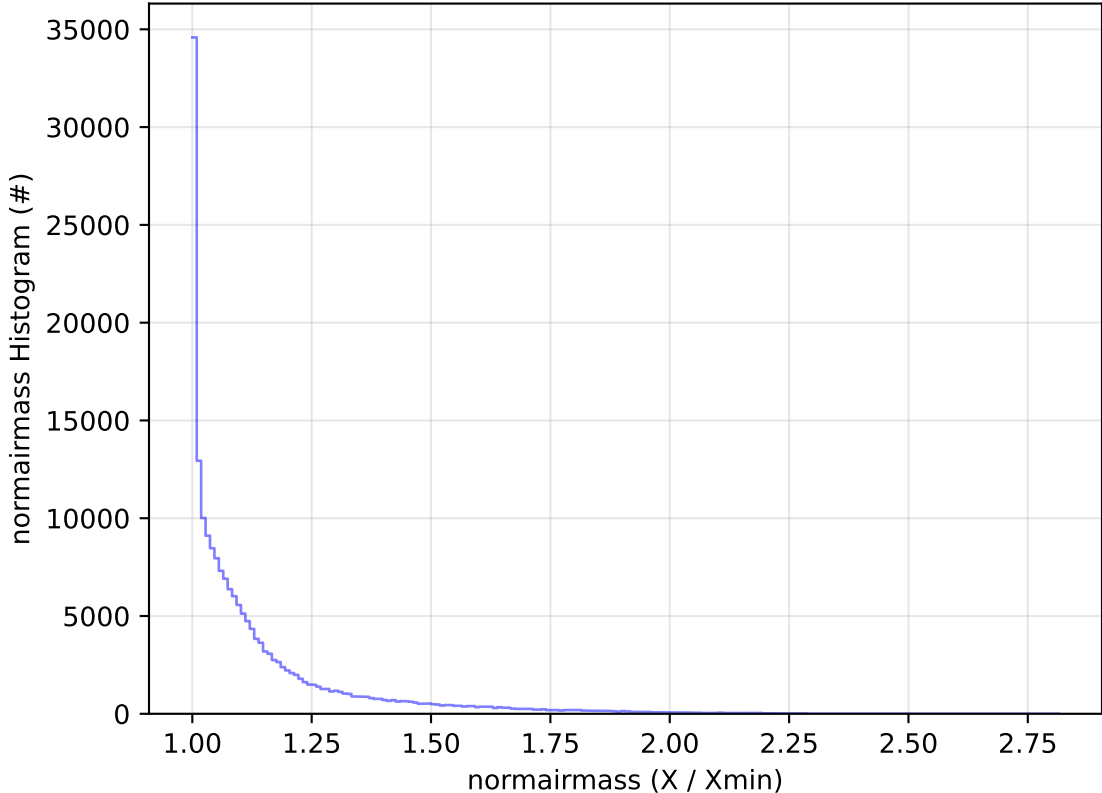
early_ss_template_fpextra2.0_v3.4_10yrs All sky g band: normairmass Histogram
