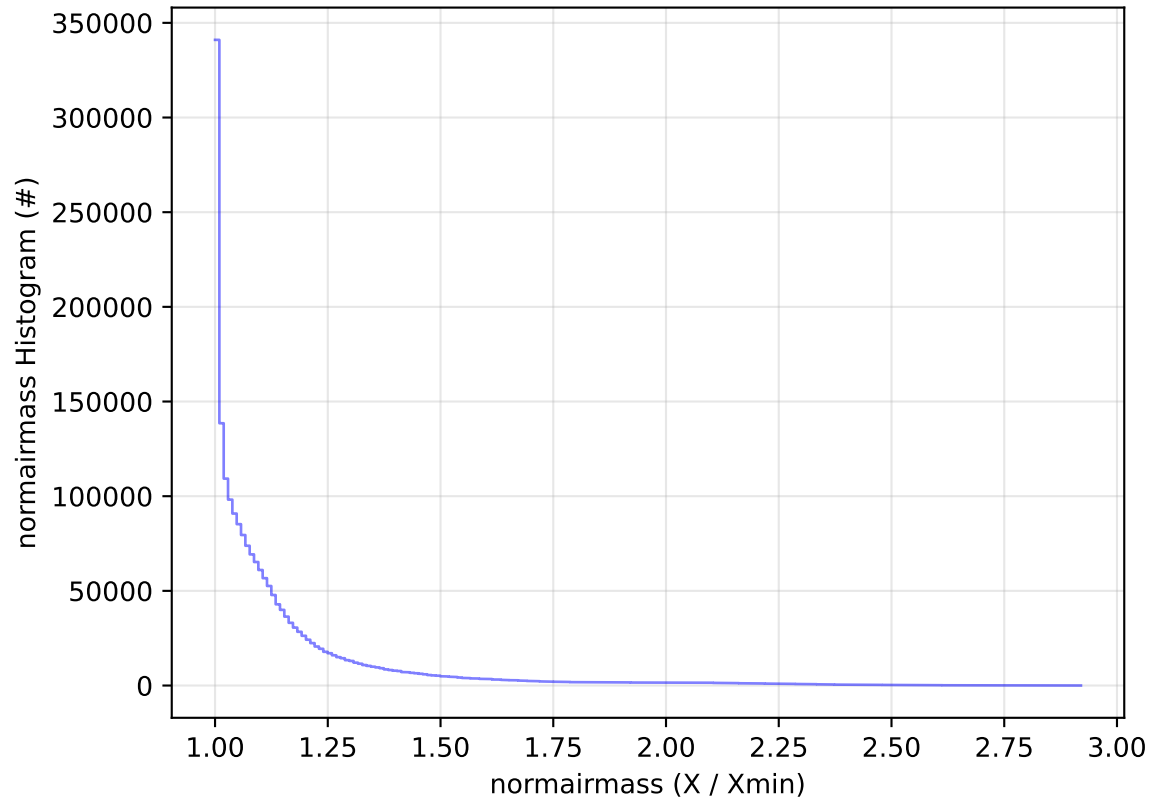
early_ss_template_fpextra2.0_v3.4_10yrs All sky all bands: normairmass Histogram
