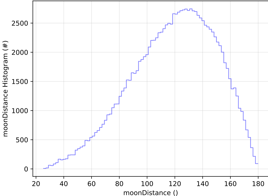
early_ss_template_fpextra2.0_v3.4_10yrs WFD u band: moonDistance Histogram
