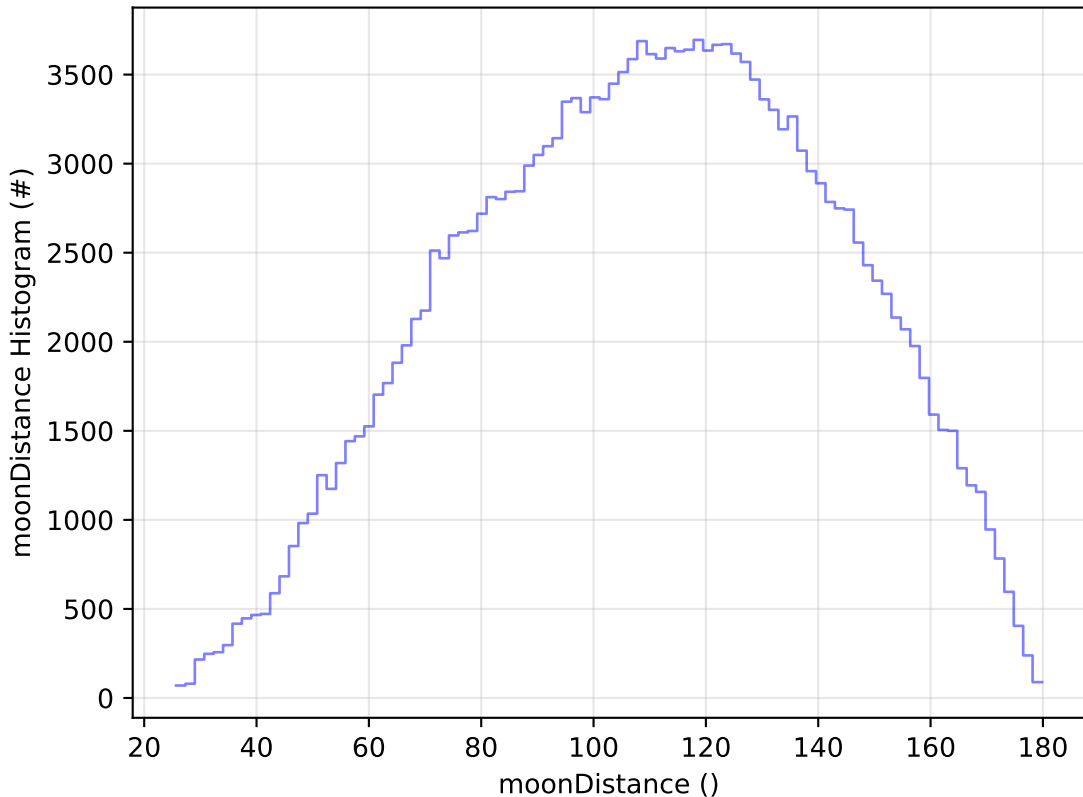
early_ss_template_fpextra2.0_v3.4_10yrs WFD g band: moonDistance Histogram
