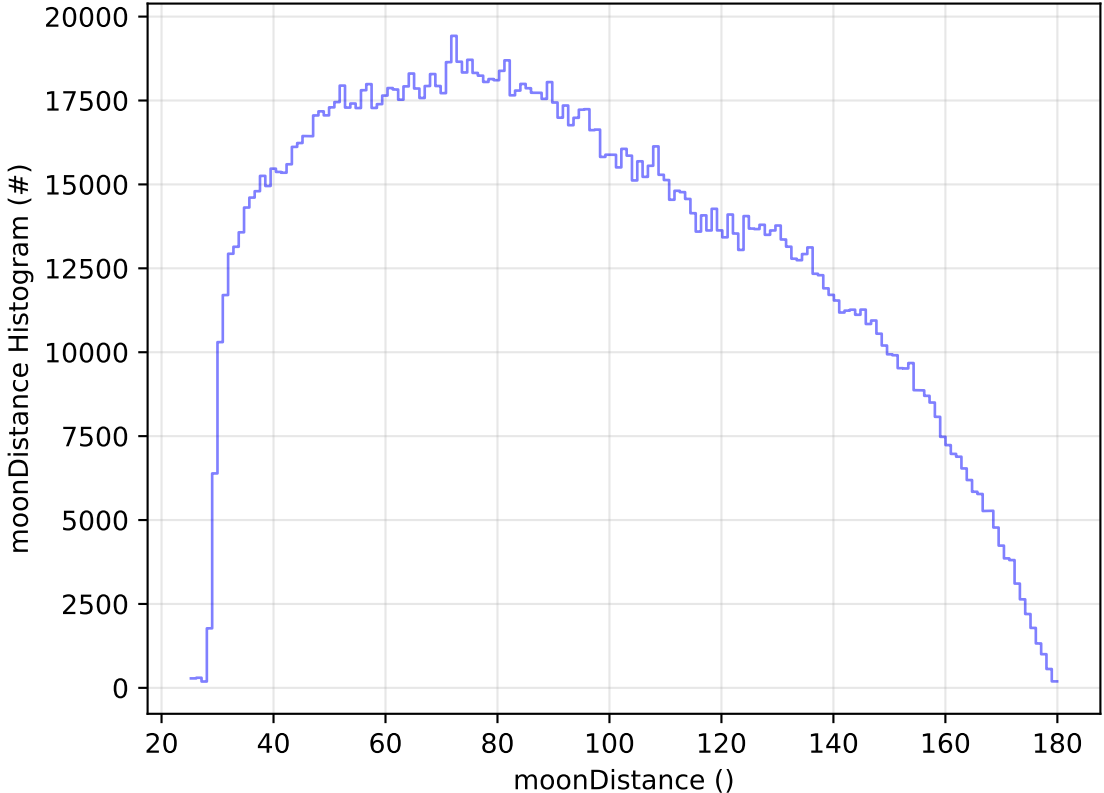
early_ss_template_fpextra2.0_v3.4_10yrs WFD all bands: moonDistance Histogram
