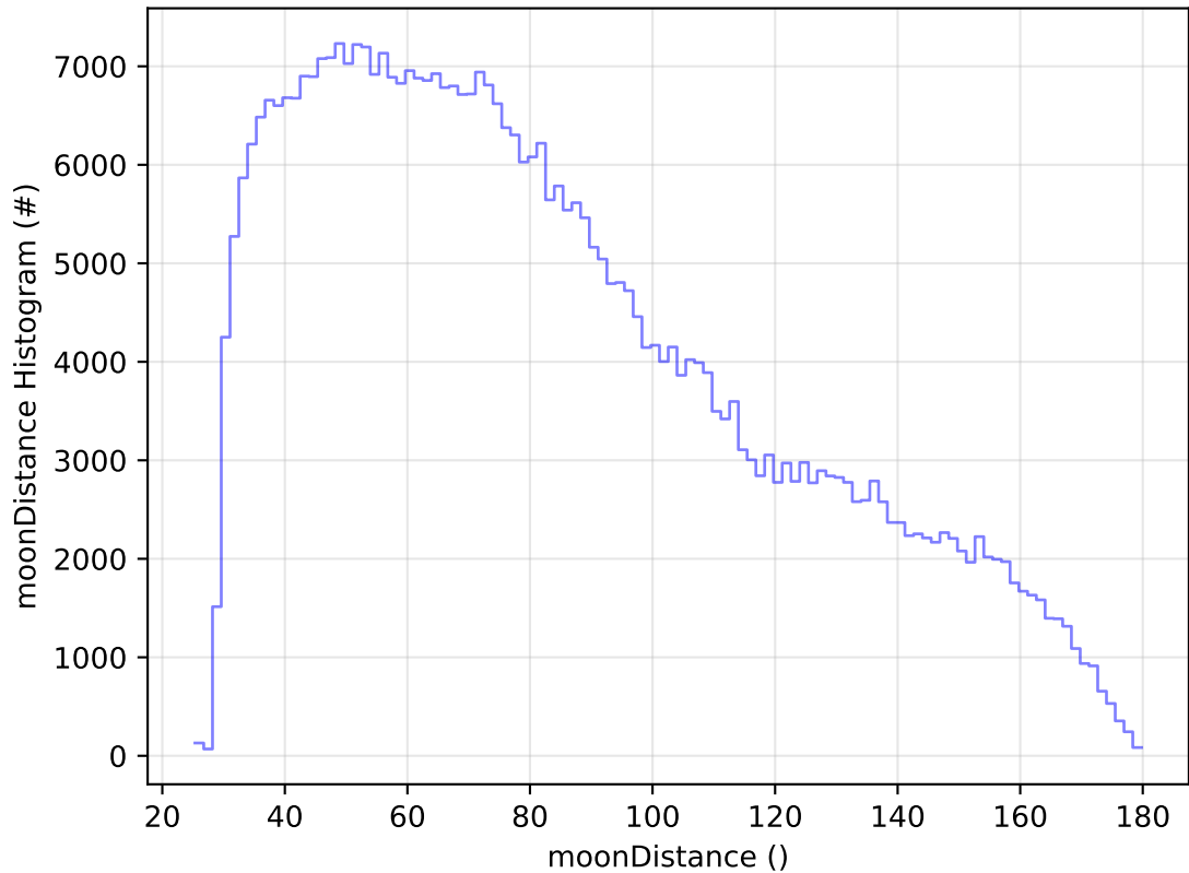
early_ss_template_fpextra2.0_v3.4_10yrs All sky z band: moonDistance Histogram
