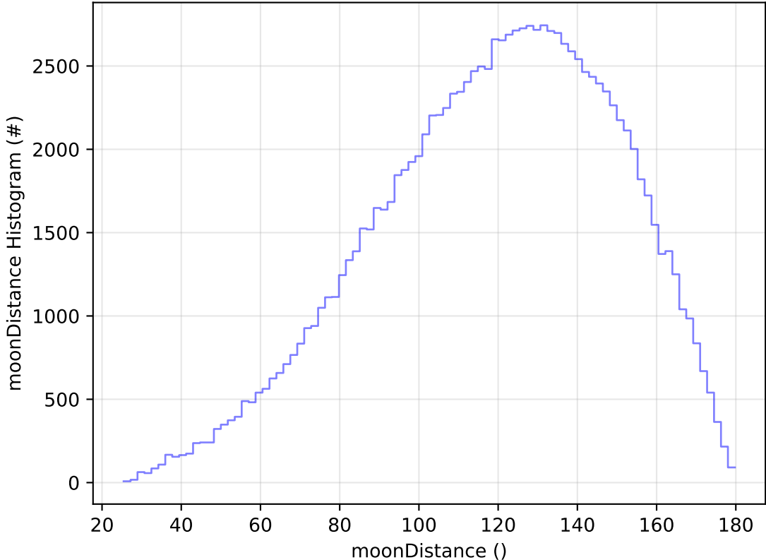
early_ss_template_fpextra2.0_v3.4_10yrs All sky u band: moonDistance Histogram
